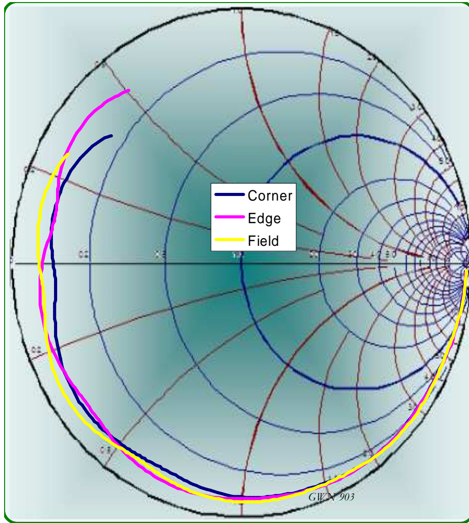
Figure 12 Reflections from the open circuited BGA contacts
