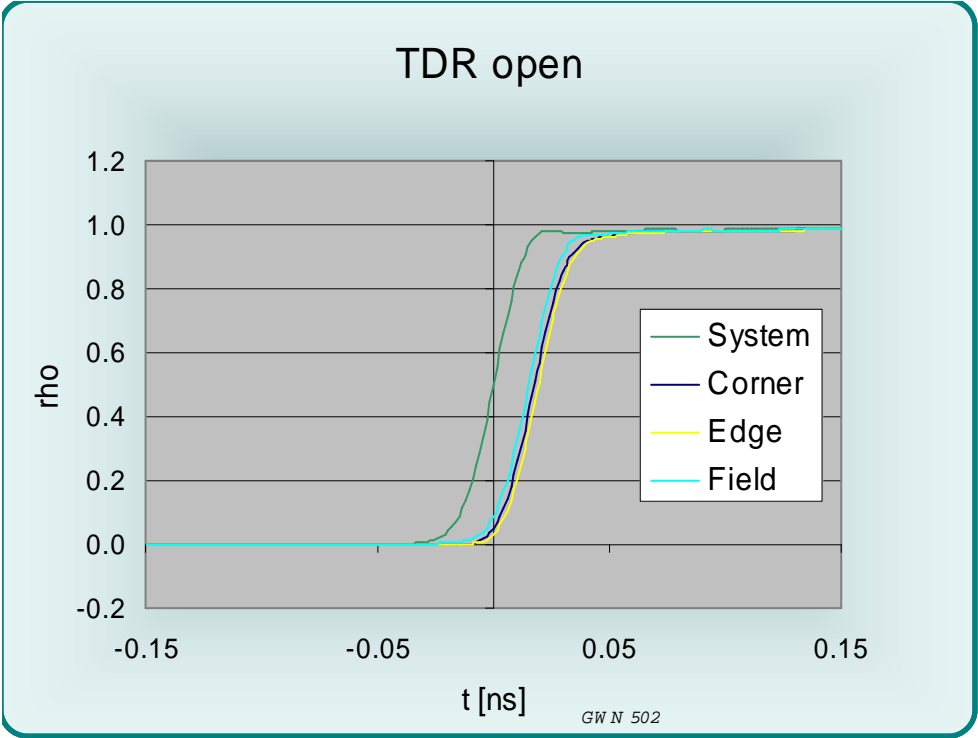
Figure 5 TDR signal from an OPEN circuited contact array
