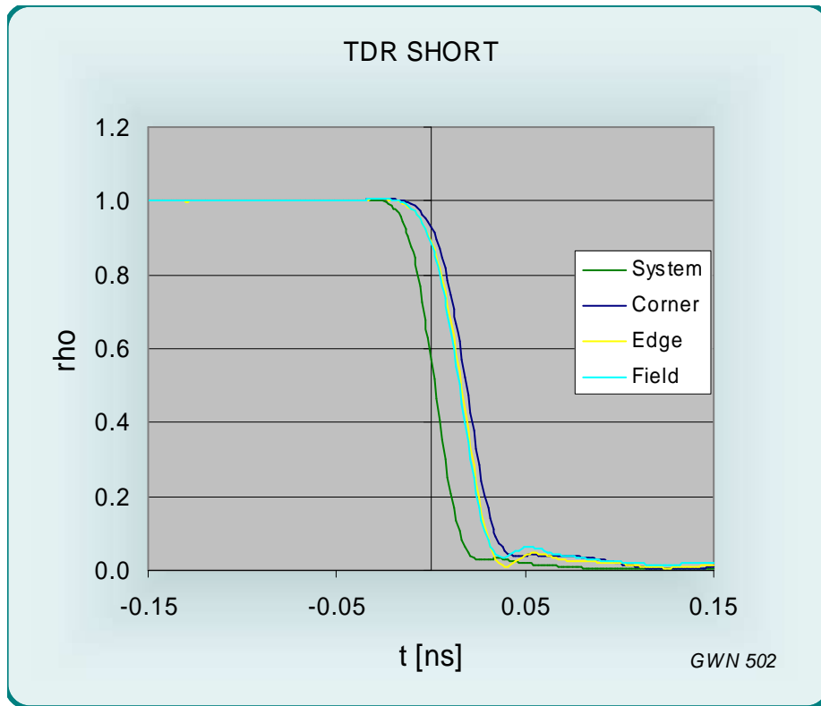
Figure 6 TDR signal from a SHORT circuited BGA array
